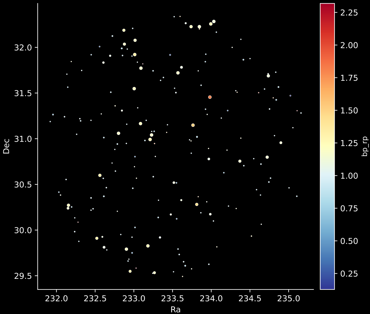
APOGEE DR17 Field: [194+39_MGA] Stars: 187
