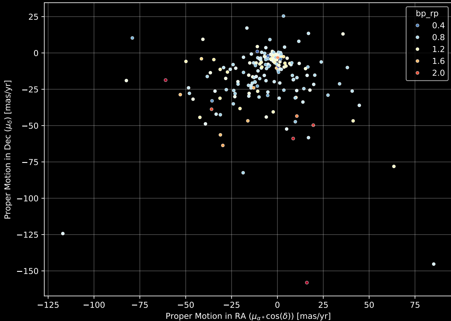
APOGEE DR17 Field: [194+39_MGA] Proper Motion Diagram (n= 187)
