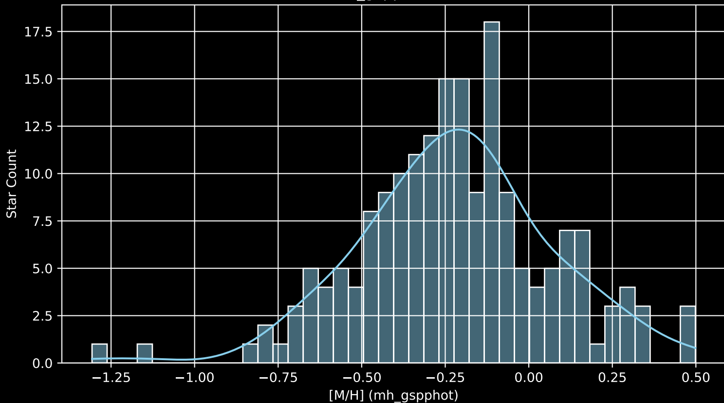
APOGEE DR17 Field: [194+39_MGA [M/H] (mh_gspphot) (n= 185)
