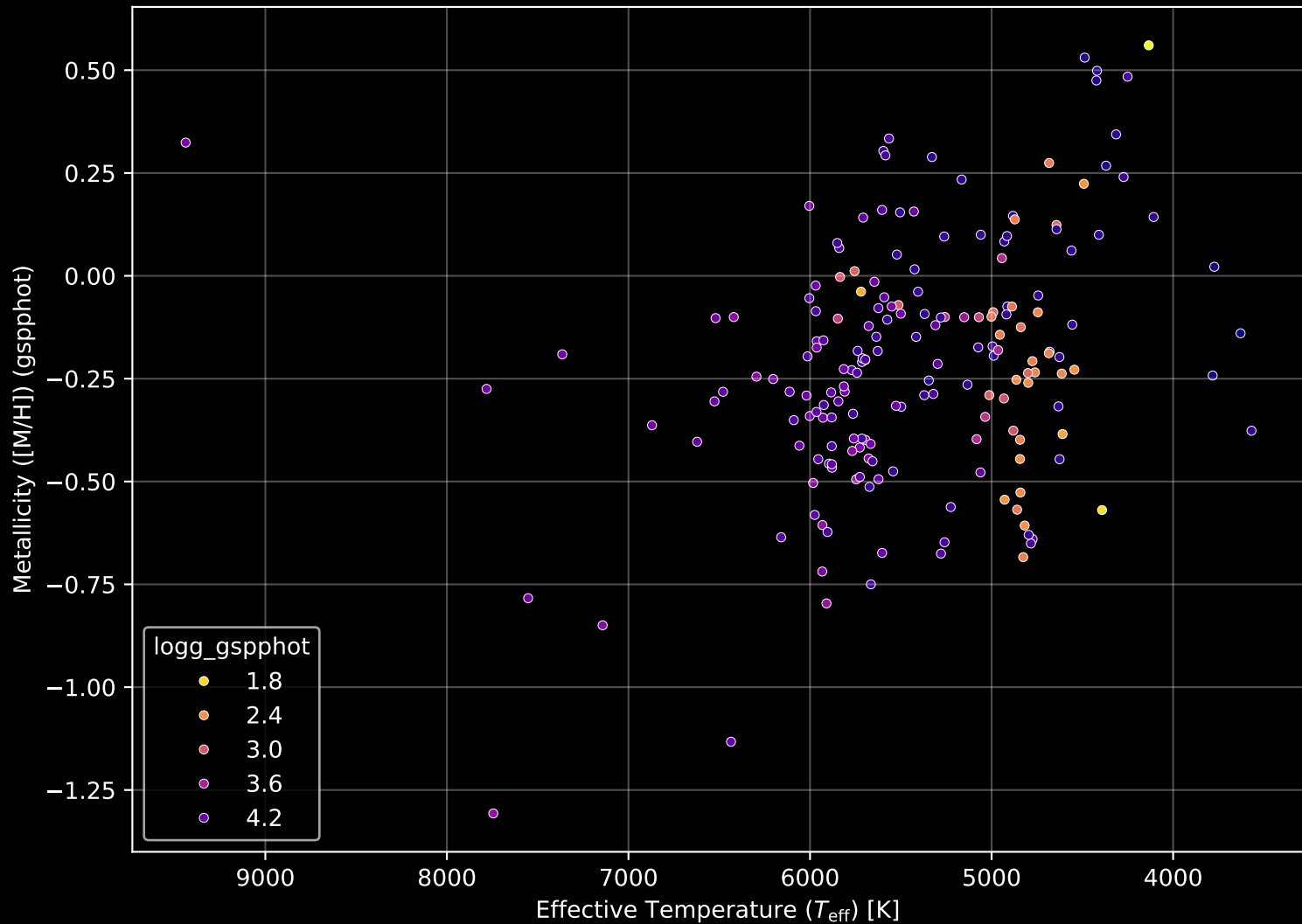
APOGEE DR17 Field: [194+39_MGA] Stellar Population Parameters (n= 187)
