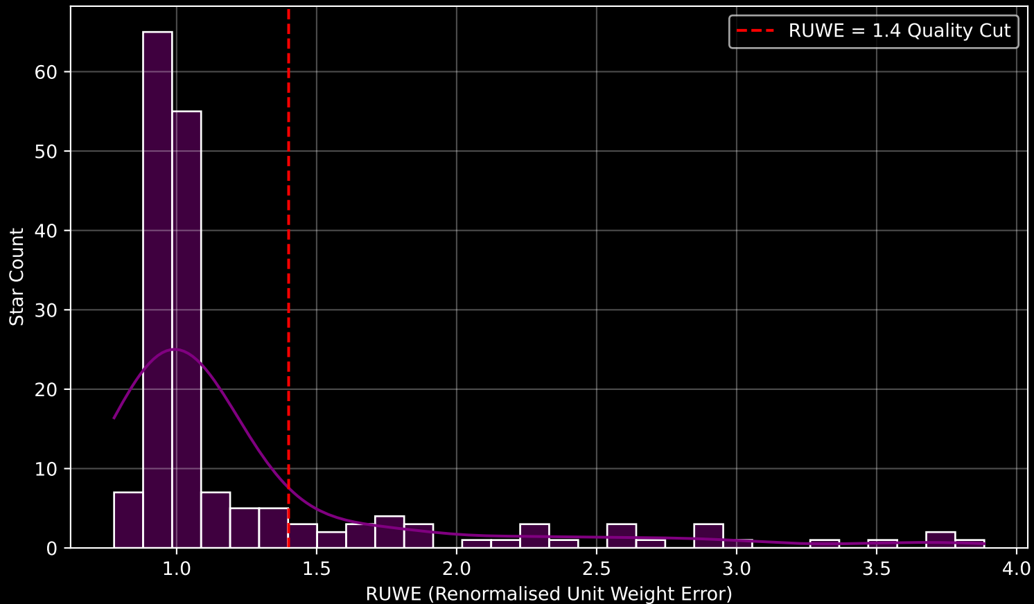
GAPOGEE DR17 Field [194+39_MGA] RUWE Distribution (n= 178)
