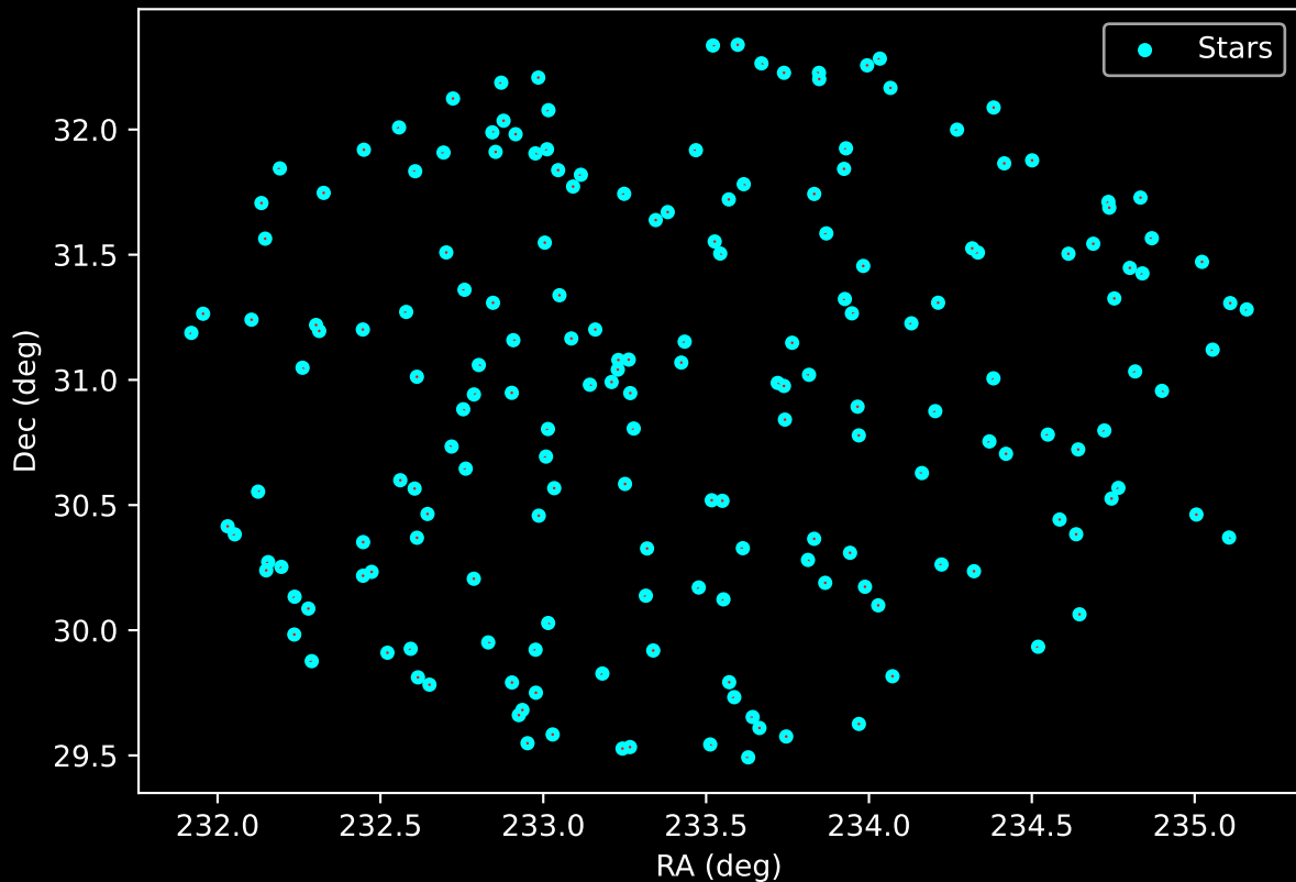
APOGEE DR17 Field: [194+39_MGA] Proper Motion Vectors for Gaia Star Field (n= 187)
