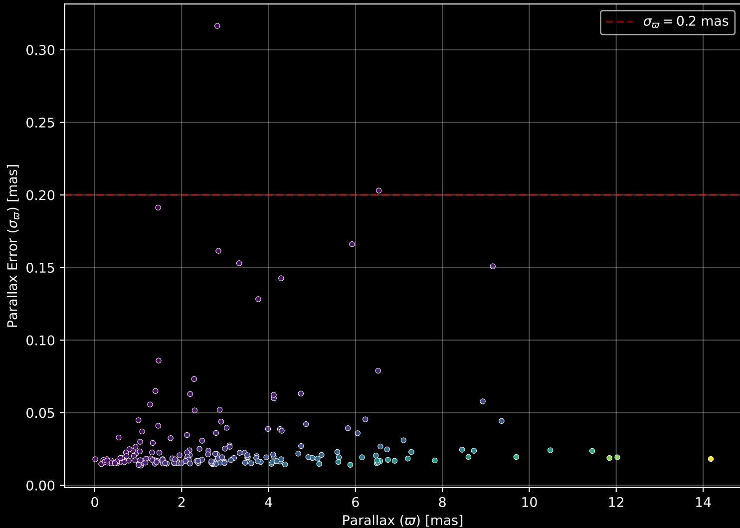
APOGEE DR17 Field: [194+39_MGA] Parallax Quality (n= 187)
