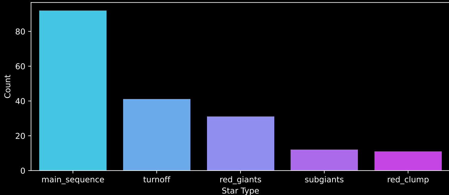
APOGEE DR17 Field: [194+39_MGA] Count plot of Star Type
